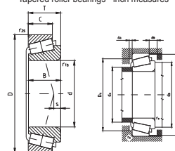
Tapered roller bearings - inch measures
